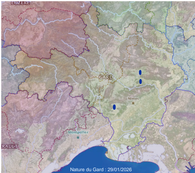
1 - Pyronia Hübner, 1819
